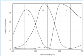
Spectral Sensitivity for G0323C
